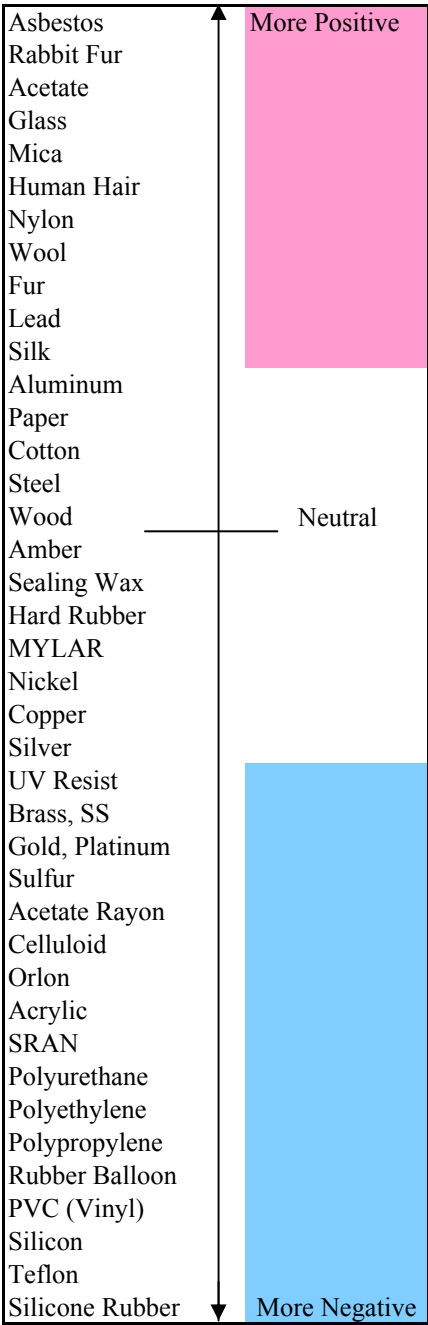
Triboelectric Series
